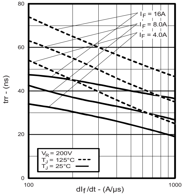
Fig. 5 - Typical Reverse Recovery Time vs. di/dt (Per Leg)
