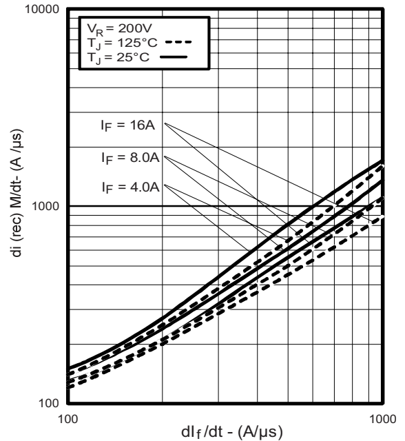
Fig. 8 - Typical di_{(rec)M}/dt vs. di/dt (Per Leg)
