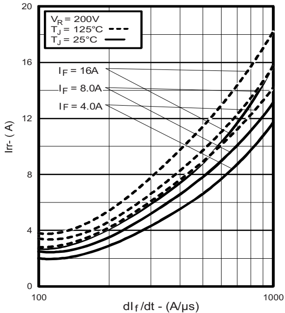
Fig. 6 - Typical Recovery Current vs. di/dt (Per Leg)
