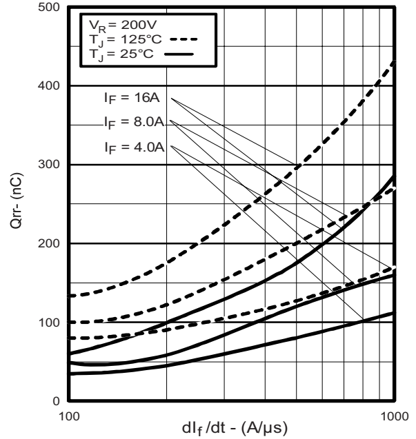
Fig. 7 - Typical Stored Charge vs. di/dt (Per Leg)
